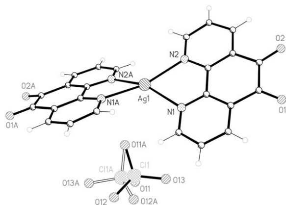
Fig. 2. X-ray crystal structure of [\text{Ag}(\text{phenidio})_2]\text{ClO}_4 .
