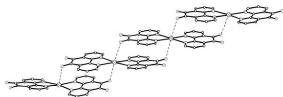
Fig. 3. Intermolecular and \pi - \pi stacking interactions in the structure of [\text{Ag}(\text{phenidio})_2]\text{ClO}_4 .
