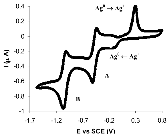
Fig. 4. Cyclic voltammogram of [\text{Ag}(\text{phendio})_2]\text{ClO}_4 .
